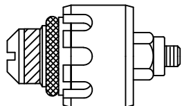
AIR CHECK ASSEMBLY P/N 11-6032A403 REPLACES P/N 10-403-32-1 QTY: 1 REFERENCE NOTE 2
